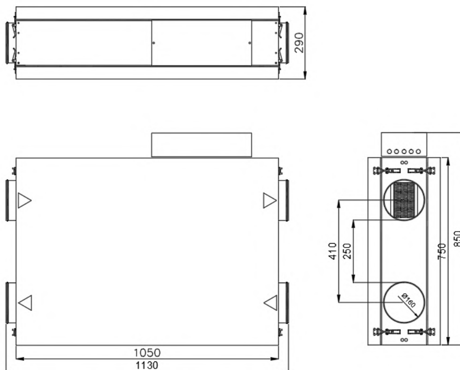
Zenit Standart 300 E
